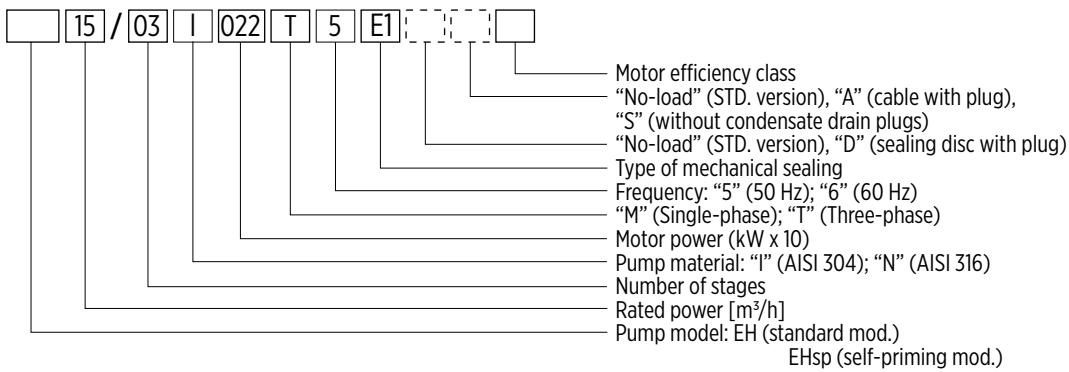
Fig. 2: Electric pump rating plate
